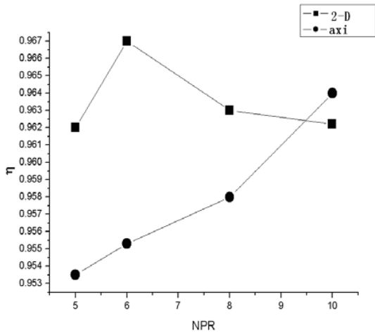
Fig. 11 The thrust coefficient comparison with different NPR ( ω=4% )
