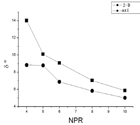
Fig. 13 The vector angle comparison with different NPR ( ω=6% )
