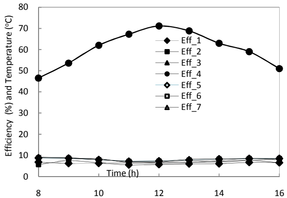
Fig. 5 Variations of panel efficiencies and panel temperature over a day at various lifting heads
