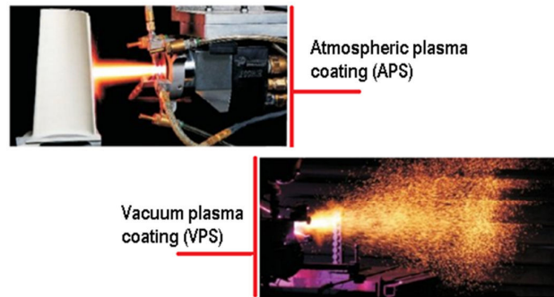
Fig. 4 Plasma coatings [8]
