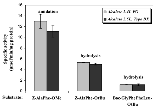
Fig. 4 Screening of proteases for the ammonolysis and hydrolysis of peptides
