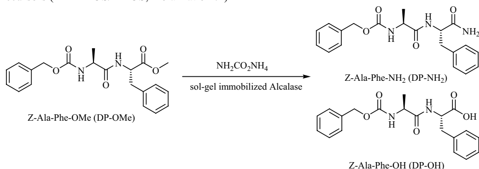
Fig 1 Reaction scheme of enzymatic synthesis of the model dipeptide amide (DP-NH 2 , dipeptide amide; DP-OH, dipeptide free acid; DP-OMe, dipeptide methyl ester; Z, benzyloxy-carbonyl protecting group)
