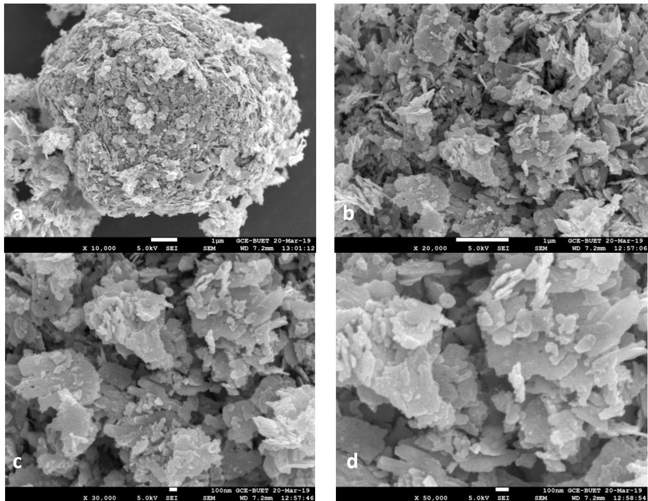
Fig. 3 SEM image of ZnO nanoparticle on different magnifications with (a) ×10000, (b) ×20000, (c) ×30000, (d) ×50000
