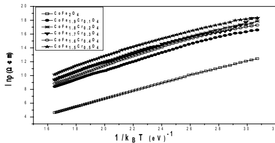
Fig. 3 Graph between resistivity ( \ln\rho ) and temperature for \text{CoFe}_{2-x}\text{Cr}_x\text{O}_4 where x=0.0, 0.1, 0.2, 0.3, 0.4, \text{ and } 0.5
