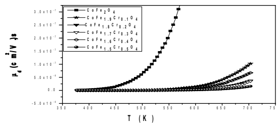
Fig.4 Graph between drift mobility ( \mu_d ) and temperature for \text{CoFe}_{2-x}\text{Cr}_x\text{O}_4 where x=0.0, 0.1, 0.2, 0.3, 0.4 \text{ and } 0.5
