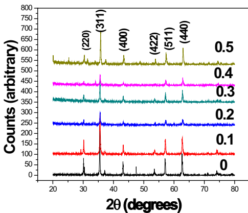
Fig. 1 XRD patterns for \text{CoFe}_{2-x}\text{Cr}_x\text{O}_4 where x=0.0, 0.1, 0.2, 0.3, 0.4, 0.5 (sintered)
