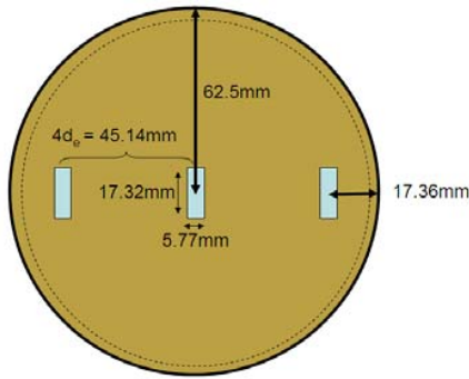
Fig. 1 Array of three parallel slot jets
