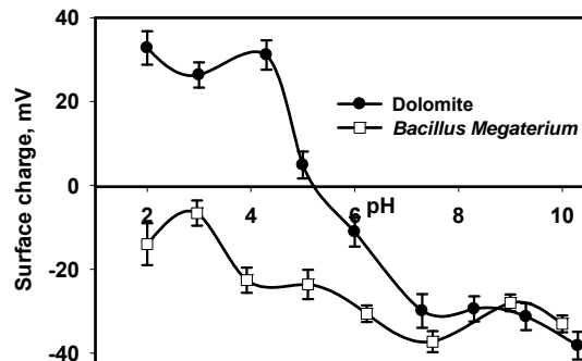
Fig. 3 Zeta potential curves for B. megaterium and dolomite, 10^{-3} M \text{KNO}_3 .
