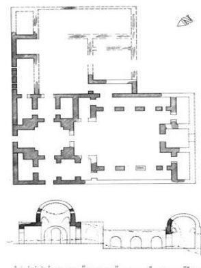
Fig.19 Plan and cross-section of “Roni” or “Rahni” building complex in Southeast of “Farashband”
