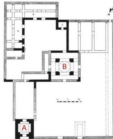
Fig.18 Plan of foundation of “Konar Siah” fire-temple (Firuz abad in Fars)
