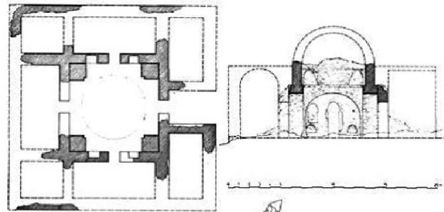
Fig.13 Plan and the cross-section of cross-vault “Kerateh” (northwest of “Duzeh” in Fars)
