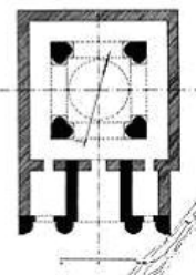
Fig.32 Exploration plan and some façades of the cross-vault “Atashkuh” (located on “Delijan-mahallat” route)
