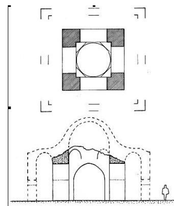
Fig.22 Exploration around Nevis-Tafrish cross-vault and the evidence to circumferential wall which made a narrow hall around square shape dome-house
