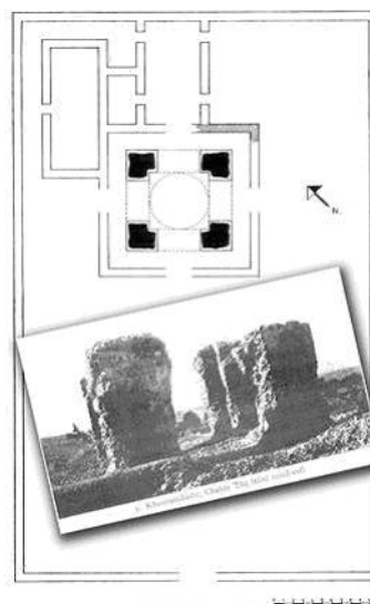
Fig.26 Plan and exploration of "Khorramdasht" cross-vault (border of "Khorramdasht" village/south of Kashan)
