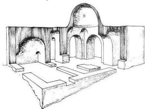
Fig.31 Cut design of “Negar” cross-vault
