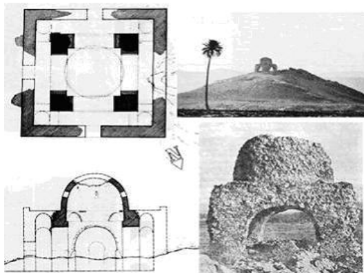
Fig.25 Plan and exploration of walls, renewed cross-section and views of "Shohrshir" (Zahrshir) cross-vault in the middle of route Fasa-Jahrom
