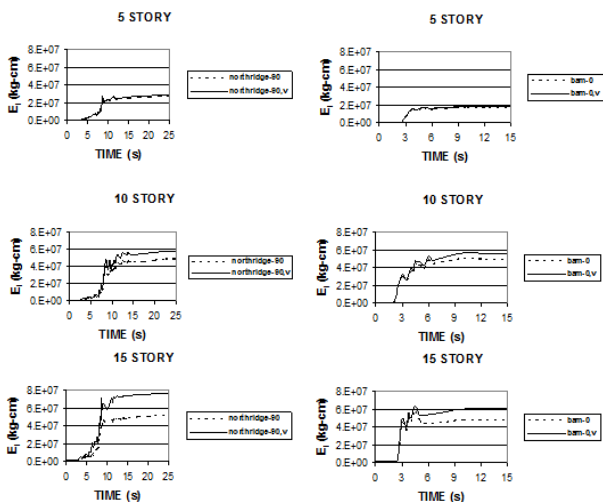
Fig. 10 Time history of input energy
