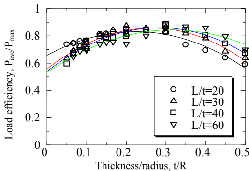
Fig. 12 Load efficiency versus t/R
