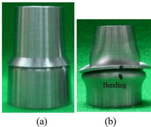
Fig. 5 Deformation of compress-expand member one
