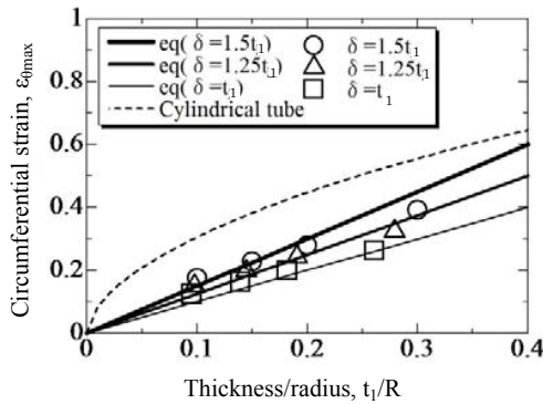
Fig. 19 \varepsilon_\theta from approximate equation and FEM
