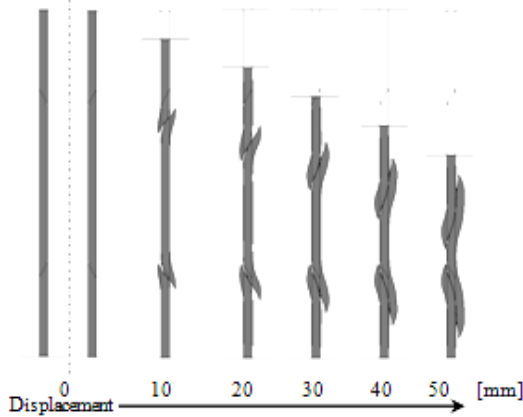
Fig. 11 Deformation diagram ( R=10 [mm], L=120 [mm], t=3 [mm])
