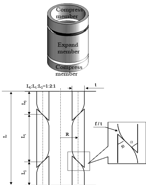
Fig. 2 Compress-expand member
