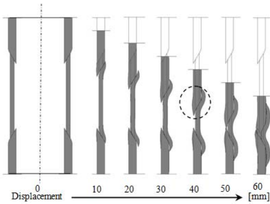
Fig. 18 Deformation diagram ( t_2=3[\text{mm}] , \delta=1.5t_2 load)
