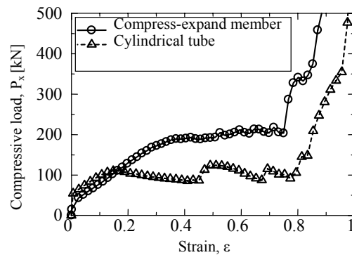
Fig. 14 Load comparison between compress-expand member and circular tube
