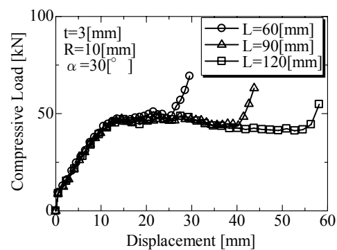
Fig. 10 Load-displacement curve for varied lengths
