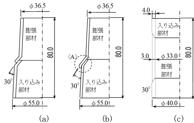
Fig. 3 Tube geometry and loading condition
