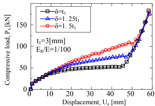
Fig. 17 Load-displacement curve with radius difference
