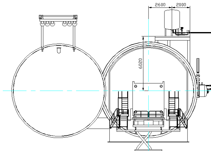
Fig. 2 (b) Layout drawing of gravity circulation loop system in left view
