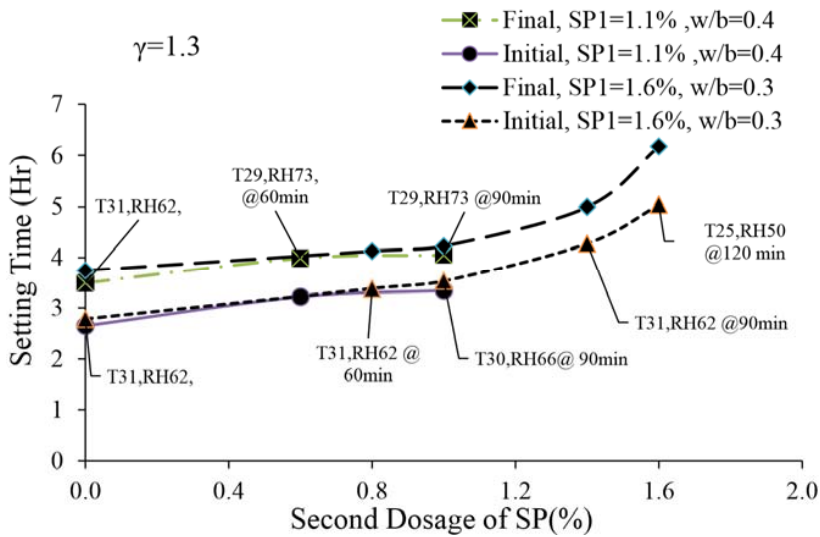
Fig. 4 Effect of second dose on setting times of low water-binder ratio OPC concrete
