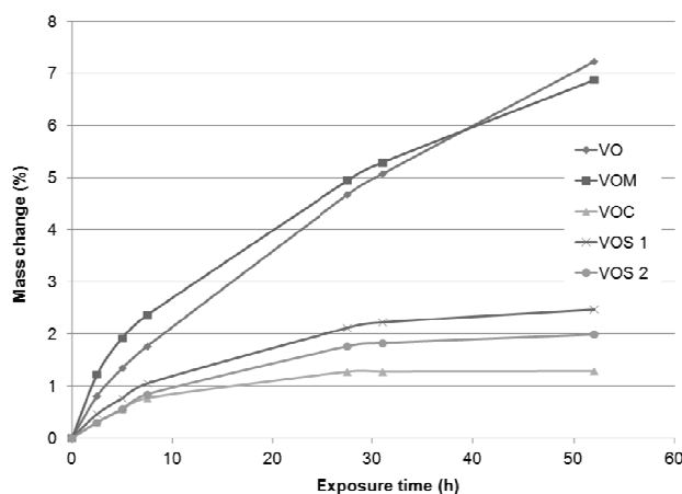
Fig. 6 The mass increase during carbonation at 5% \text{CO}_2 concentration
