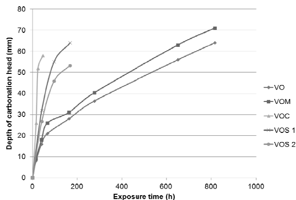
Fig. 4 The depth of carbonation head at 5% \text{CO}_2 concentration
