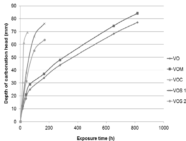
Fig. 5 The depth of carbonation head at 10% \text{CO}_2 concentration
