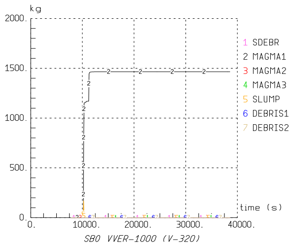
Fig. 27 ASTECv2 SBO with actuation one HPP at 14000s; Corium Mass in the Lower Plenum
