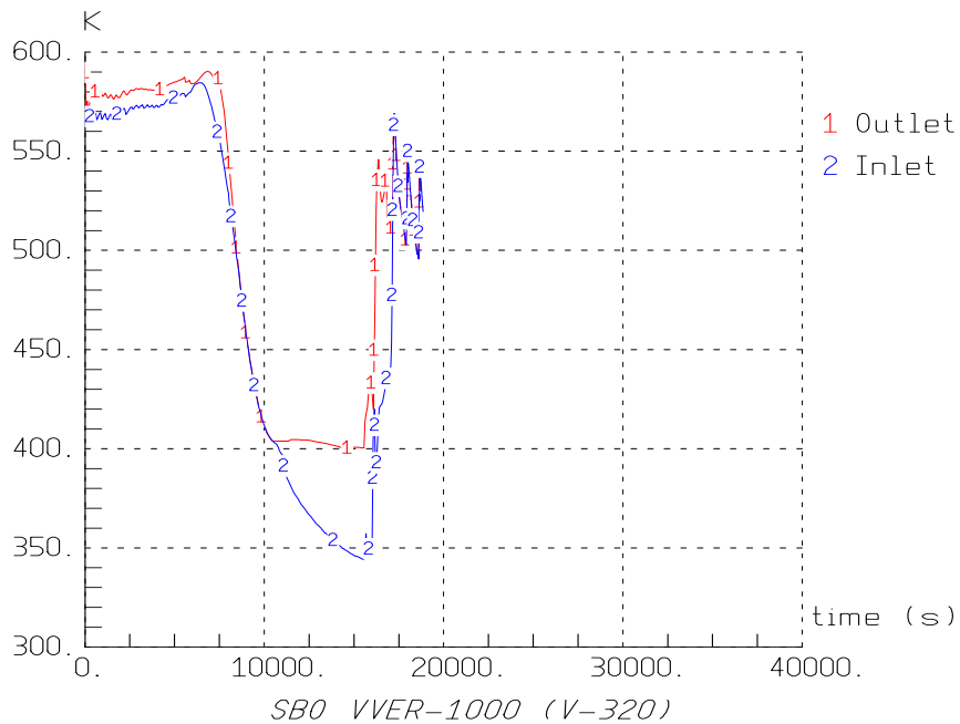
Fig. 8 ASTECv2 SBO with actuation one HPP at 16000s; Reactor Inlet &amp; Outlet Temperatures
