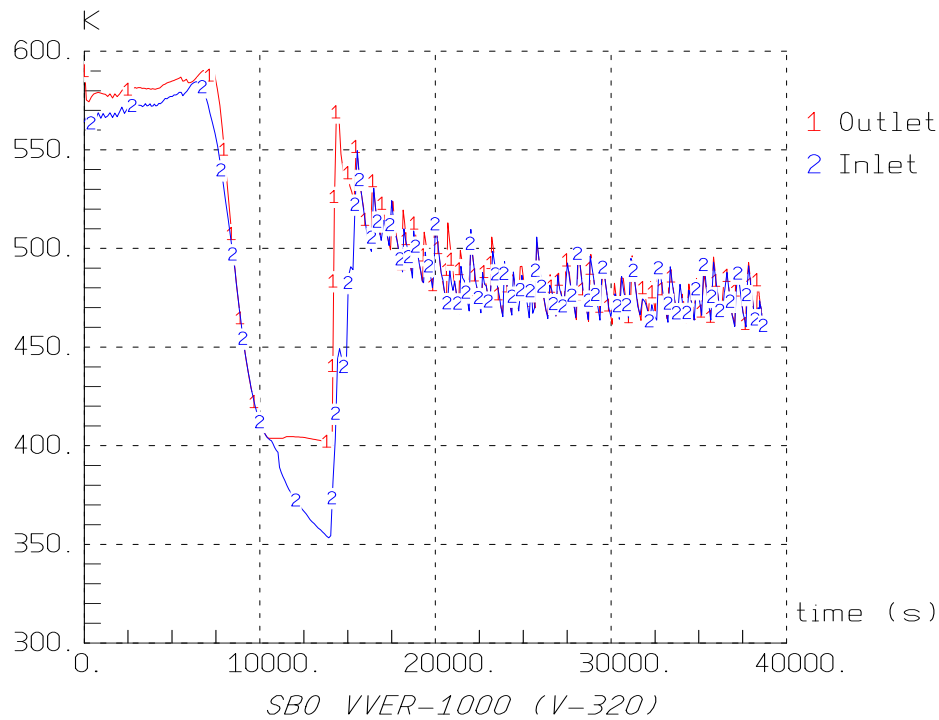
Fig. 7 ASTECv2 SBO with actuation one HPP at 14000s; Reactor Inlet &amp; Outlet Temperatures
