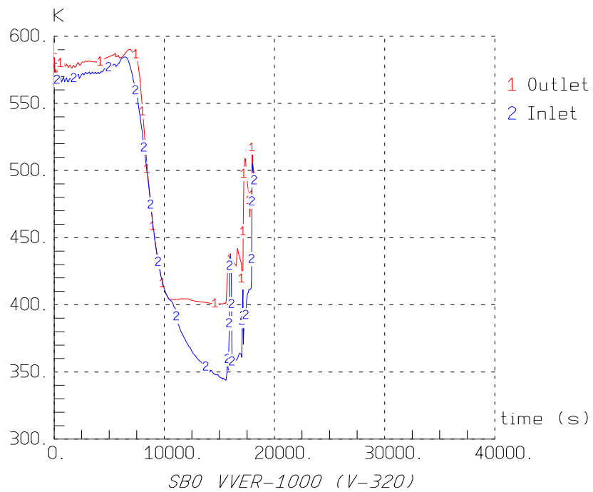
Fig. 9 ASTECv2 SBO with actuation one HPP at 17000s; Reactor Inlet &amp; Outlet Temperatures
