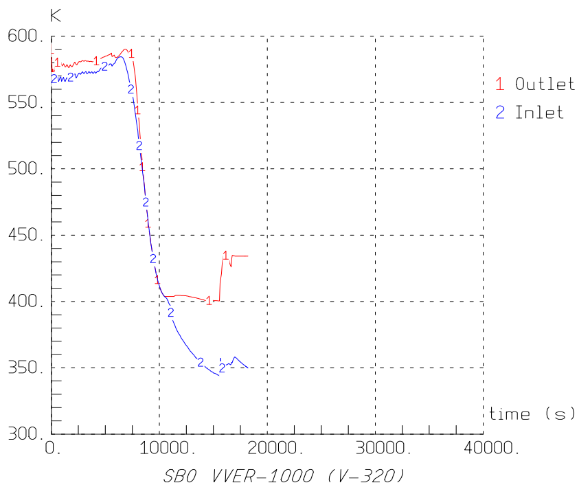
Fig. 10 ASTECv2 SBO without HPIS actuation; Reactor Inlet &amp; Outlet Temperatures
