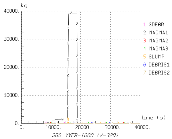
Fig. 28 ASTECv2 SBO with actuation one HPP at 16000s; Corium Mass in the Lower Plenum
