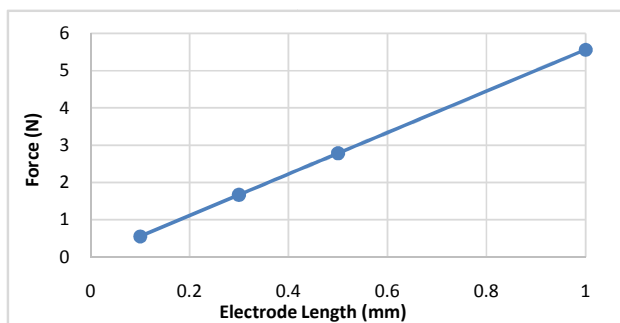
Fig. 12 Attraction force compared to the electrodes length
