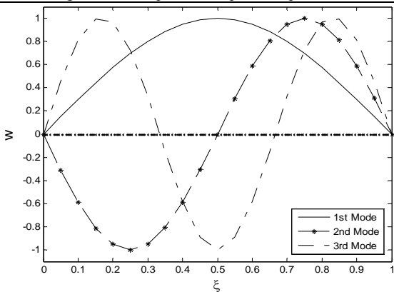
Fig. 3 Mode shapes of clamped-clamped beam
