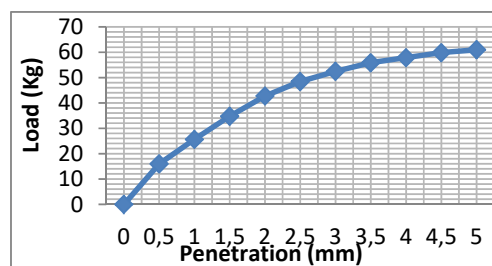
Fig. 3 Load penetration curve
