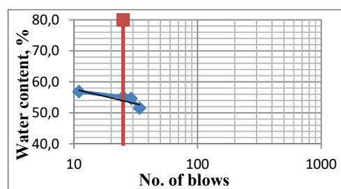
Fig. 2 Flow curve
