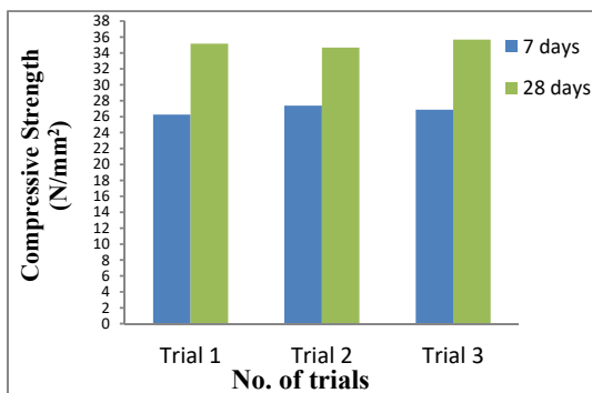
Fig. 6 Compressive strength results
