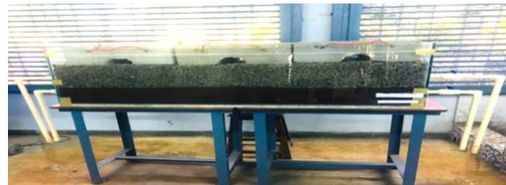
Fig. 8 Permeable articulating concrete blocks model
