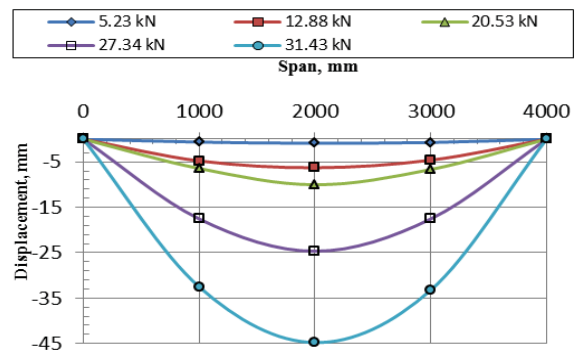
(b) Deflection against span for panel GF6
