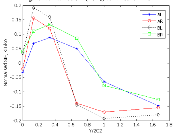
Fig. 18 Normalized SIF ( K_{II}/K_0 ) vs Y/2C_2 for H=5
