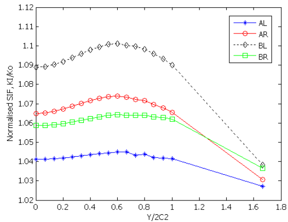
Fig. 7 Normalized SIF ( K_I/K_0 ) vs Y/2C_2 for H=15
