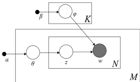
Fig. 1 Graphical model representation of LDA. The boxes are plates representing replicates and the outer plate represents documents, and the inner plate represents the repeated choice of topics within a document
