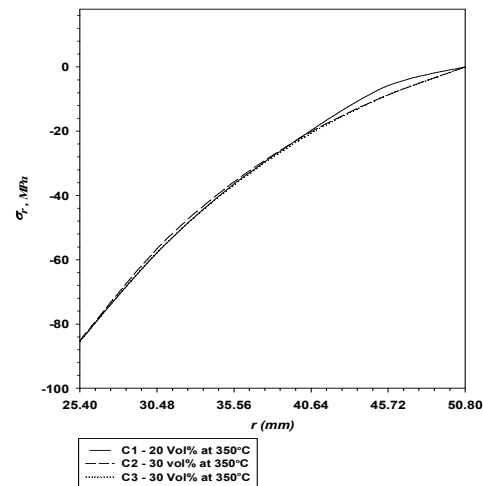
Fig. 5 Distribution of radial stress
