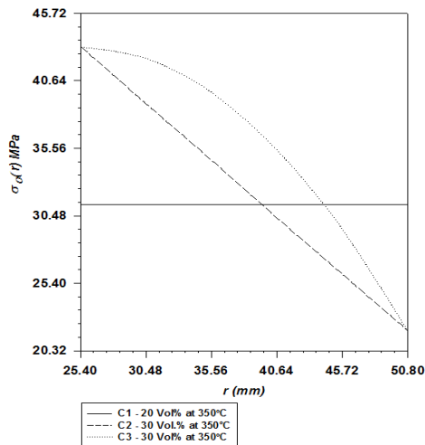
Fig. 4 Distribution of Creep Parameters \sigma_0(r)
