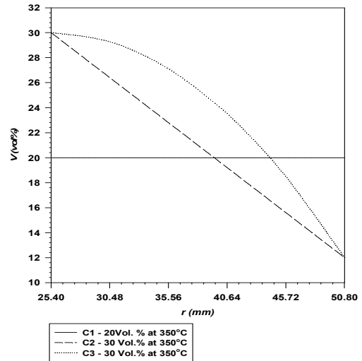
Fig. 2 Distribution of reinforcement
