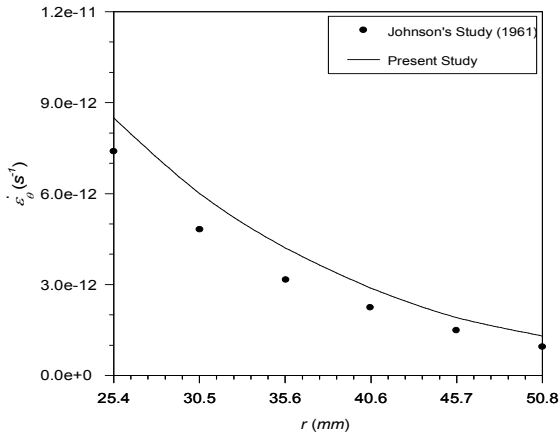
Fig. 1 Comparison of tangential strain rates
