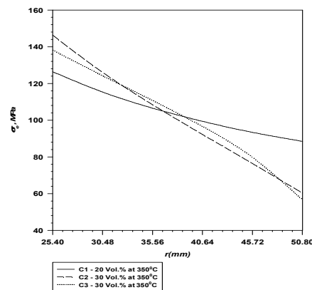
Fig. 8 Distribution of effective stress
