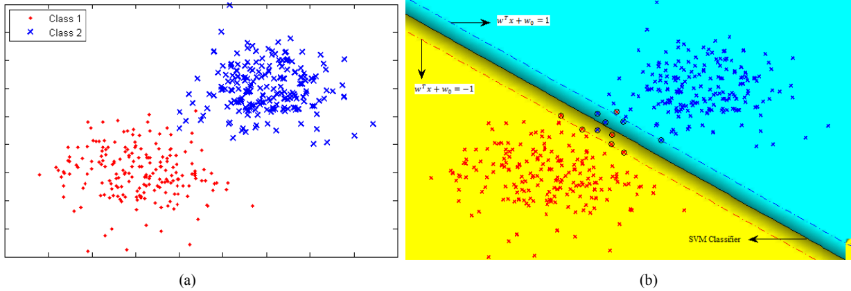
Fig. 3 (a) Distribution of 2-dimensional data set of two different classes (b) Support vectors (dotted lines) and SVM classifier (solid line) learnt to optimize for minimum training error and maximum separating margin between hyper-planes
