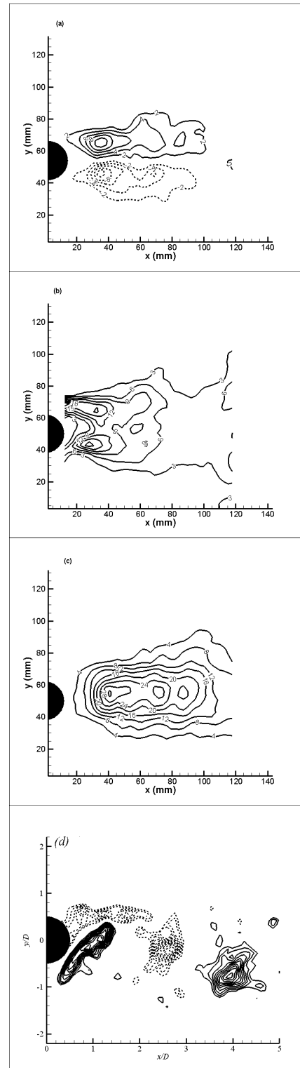
Fig. 2 Reynolds stress distributions in the x - y plane for \lambda = 0 (a) -\overline{uv}/U_\infty^2 \times 100 (b) \overline{u^2}/U_\infty^2 \times 100 (c) \overline{v^2}/U_\infty^2 \times 100 (d) instantaneous vorticity contours
