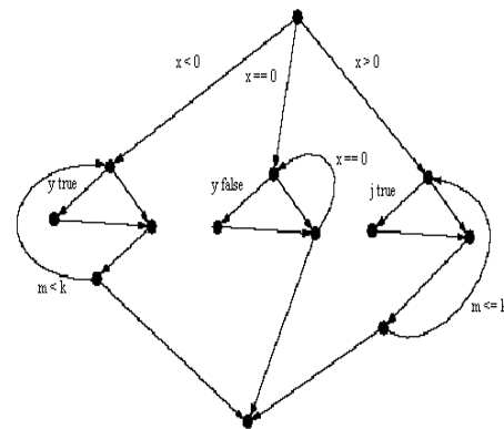
Fig. 1 Flowgraph of the Example Program
