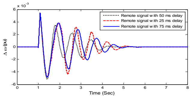
Fig. 14 Speed deviation response showing for case-IV
