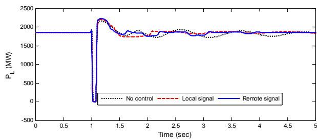
Fig. 18 Tie line power flow for self clearing three phase fault disturbance
