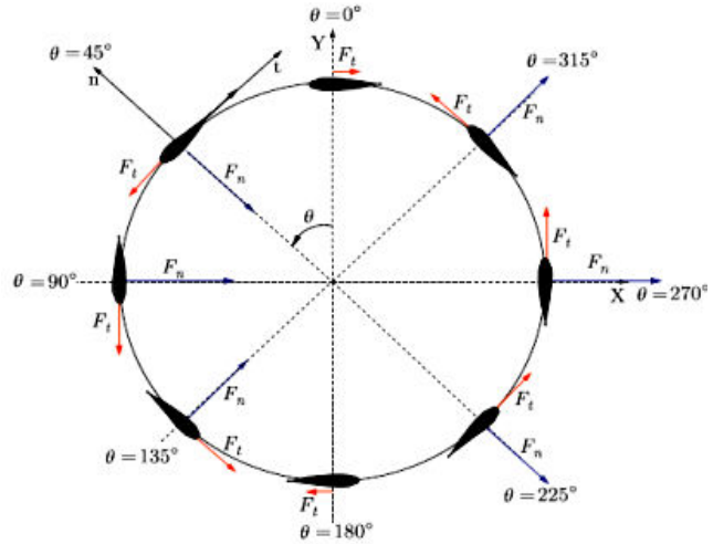
Fig. 6 Normal and tangential forces
