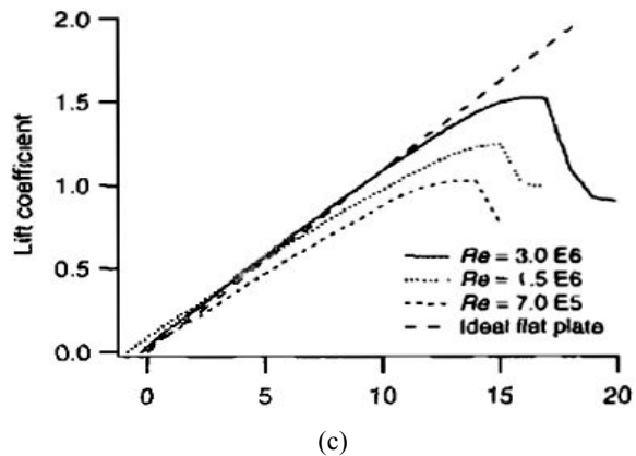
Fig. 2 Lift coefficient versus angle of attack degrees for different Re [17]
