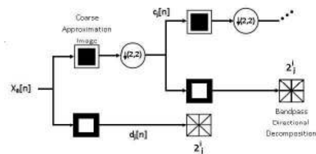
Fig. 2. The flow diagram of the contourlet transform.
