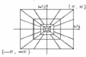
Fig. 4. Pyramidal directional decomposition. As the scale is refined from coarse to fine, the number of directions is doubled at every other subband.
