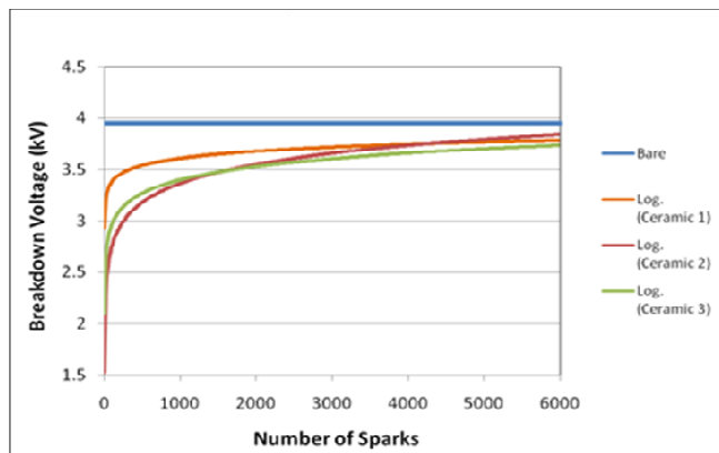
Fig. 11 Durability of MWCNT/ceramic mix over 6000 sparks
