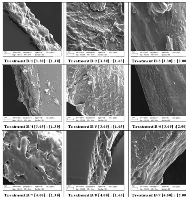
Fig. 3 SEM micrographs( 1000x ) of yam starch films
