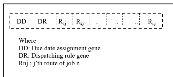
Fig. 1 Sample chromosome
