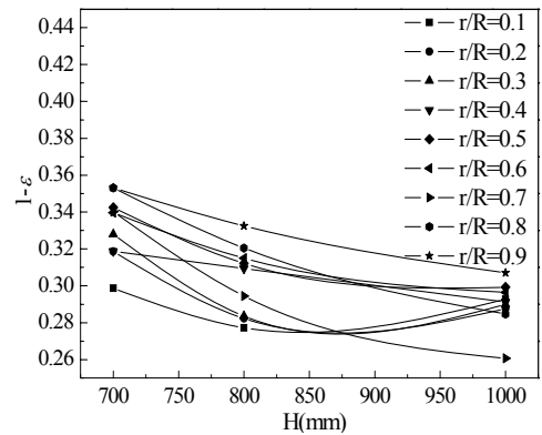
Fig. 6 H_0=800\text{mm} , U_s=0.6877\text{m/s} , Branched pipe distributor (5%)
