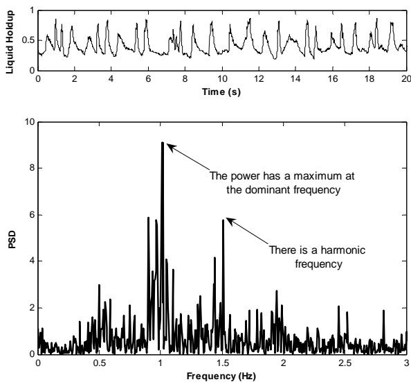
Fig. 3 Example of PSD (at the bottom) obtained from the corresponding time series (at the top) for 40° inclination, U_{SG}=0.9 m/s and U_{SL}=0.7 m/s
