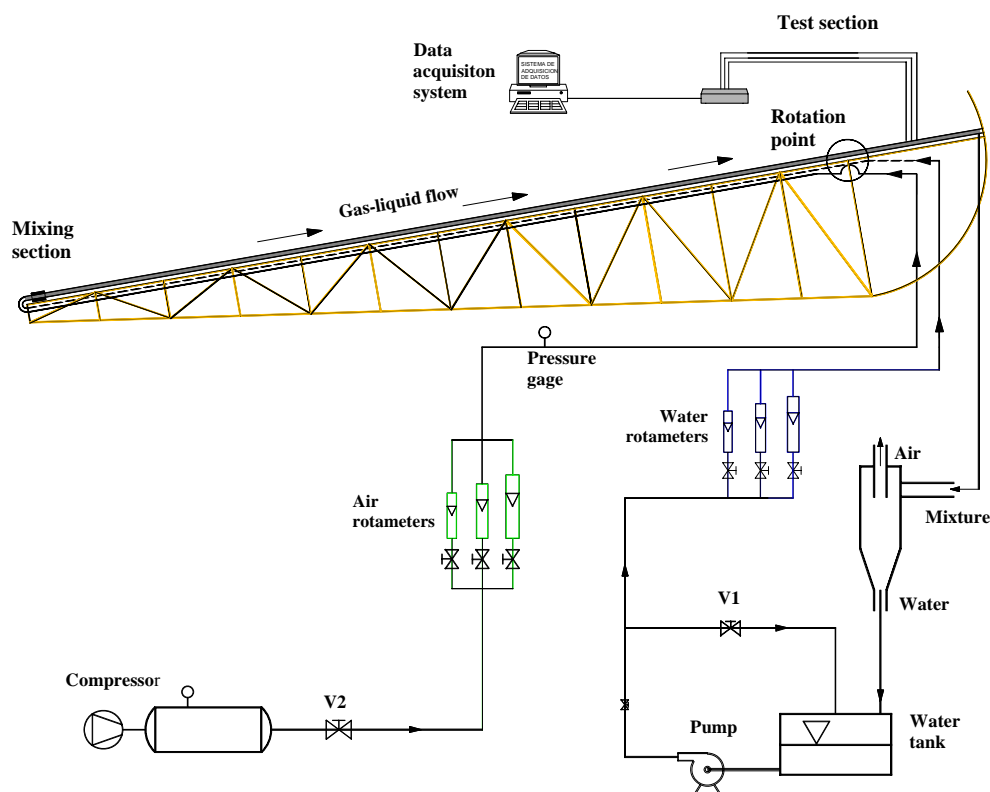
Fig. 1 Schematic diagram of inclinable rig
