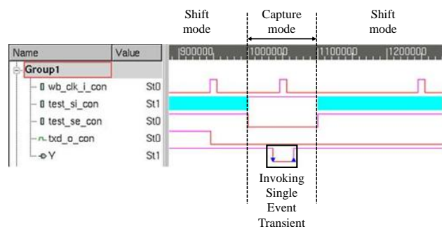
Fig. 6 Waveform of the SET
