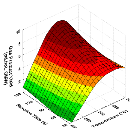
Fig. 4 The change of gas product yield with temperature and reaction time, for Ni/Al 2 O 3 catalyst
