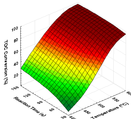
Fig. 5 The change of TOC conversion with temperature and reaction time, for Ni/Al 2 O 3 catalyst
