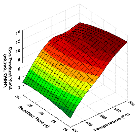
Fig. 10 The change of gas product yield with temperature and reaction time, for Pt/Al 2 O 3 catalyst
