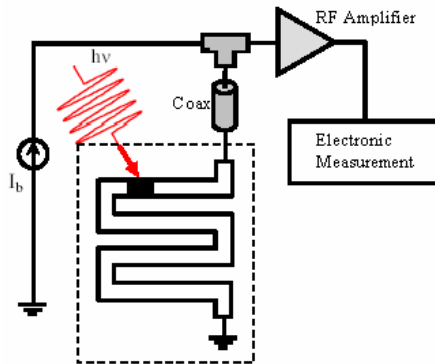
Fig. 3 Driving and measurement circuit
