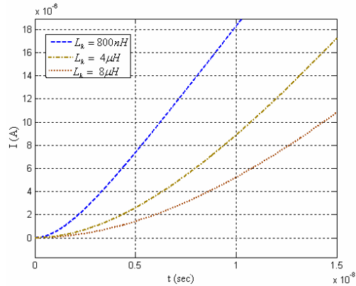
Fig. 6 The calculated current through the wire, in this curve R_n \cong 400\Omega , L_k = 800nH, 4,8\mu H are assumed
