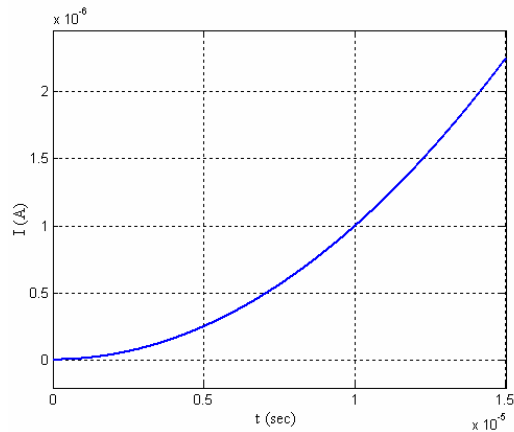
Fig. 8 The calculated current through the wire, in this curve R_n \cong 400\Omega , L_k = 800nH, 4,8\mu H are assumed
