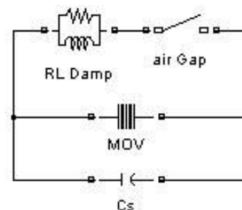
Fig. 1 MOV protection scheme for series capacitors
