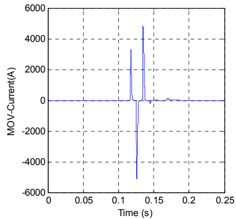
Fig 4 MOV-current
