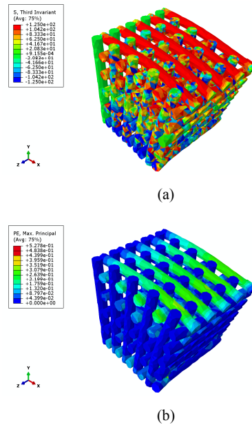
Fig. 8 Cantors of 3D orthogonal carbon fabric model applied to bending moment: (a) Stress, (b) Plastic strain
