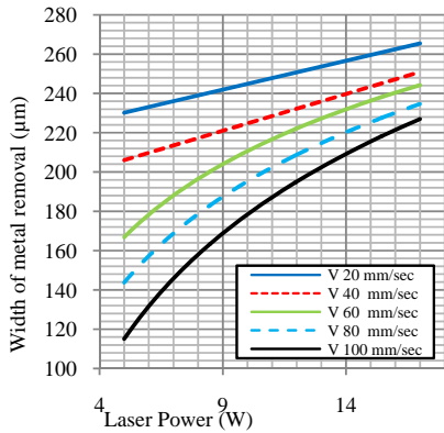
(a) The effect of the laser power on the width of the metals surface removal
