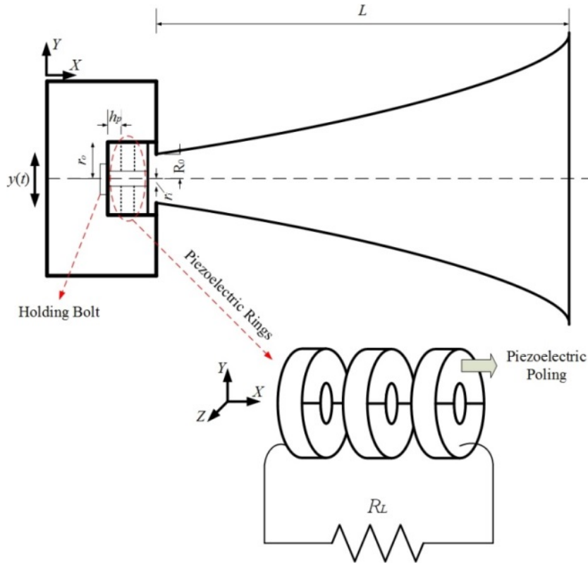
Fig. 1 Piezoelectric energy harvester with piezoelectric stacks
