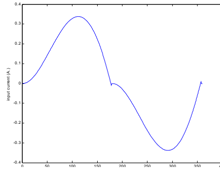
Fig. 7 Simulated input supply current
