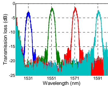
Fig. 3 Measured transmission spectra of the standing alone 1 x 4 concave grating. The transmission band wavelengths locate at 1531, 1551, 1571, and 1591 nm
