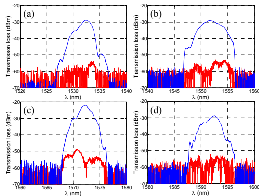
Fig. 5 The measured transmission spectra for all four channels at on/off status. (a) channel 1 at 1531 nm. (b) channel 2 at 1551 nm. (c) channel 3 at 1571 nm. (d) channel 1 at 1591 nm.
