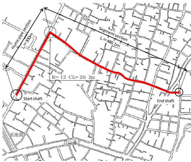
Fig. 8 Construction line
