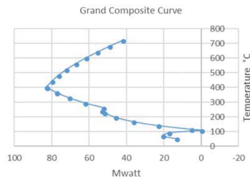
Fig. 7 Grand composite curve
