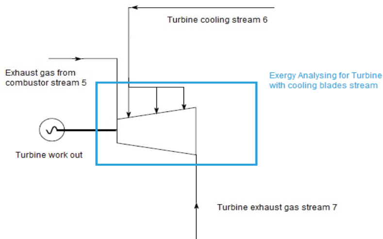
Fig. 4 NetPower Turbine with cooling blade
