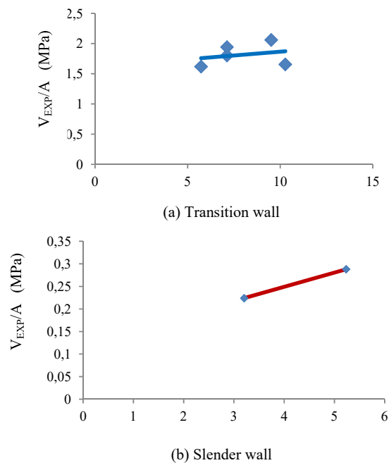
Fig. 6 Variation of ultimate shear strength with the product of boundary element reinforcement ratio and boundary element yield stress reinforcement
