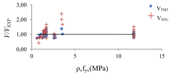
Fig. 9 Variation of the ratio V_{TM2}/V_{EXP} and V_{NTC}/V_{EXP} with the product of vertical reinforcement ratio and the vertical reinforcement yield stress \rho_V f_V (MPa)
