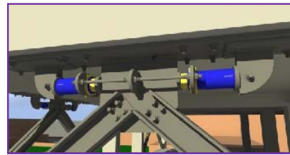
Fig. 4 Basic installation layout of FV spring-dampers designed for the Bisignano building
