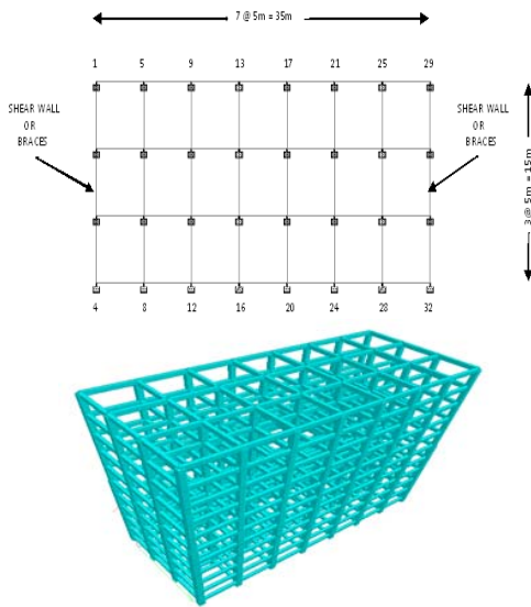
Fig. 1 Plan and isometric view of buildings
