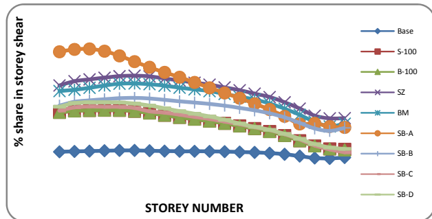
Fig. 4 Share of two exterior frames in storey shear in 20 storey buildings
