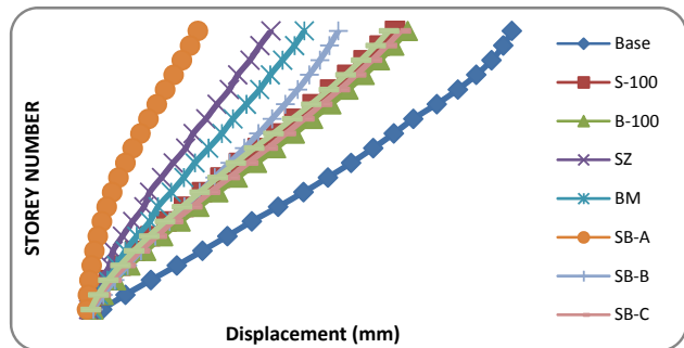
Fig. 7 Lateral displacement of end frames of 20 storey buildings
