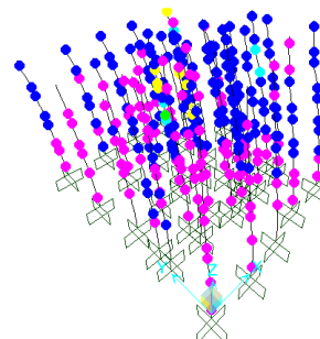
Fig. 13 (a) Model I (no infill)
