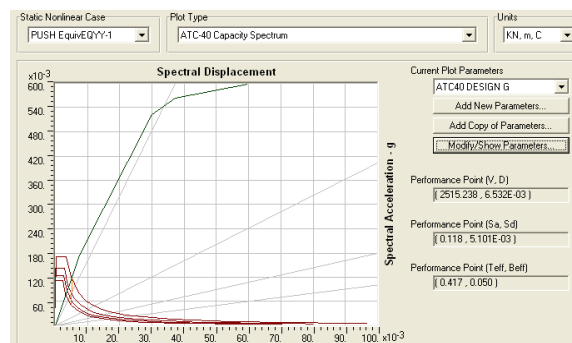
Fig. 17 (c) Model IIB (strut infill- ASCE/SEI 41), R=3.92
