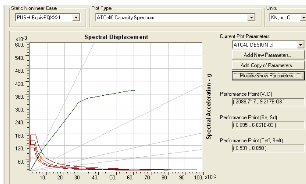
Fig. 16 (c) Model IIB (strut infill- ASCE/SEI 41), R=2.51
