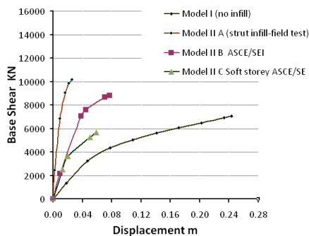
Fig. 14 (a) Static nonlinear analysis X-X
