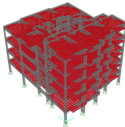
Fig. 9 Model I (no infill)
