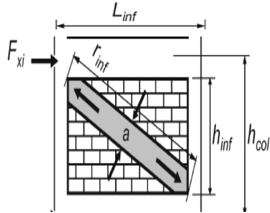
Fig. 4 Compression strut analogy—concentric Struts, ASCE/SEI 41[7]
