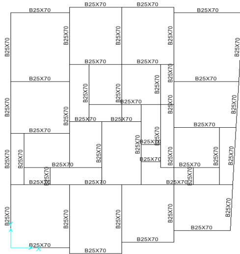
Fig. 7 Typical Plan
