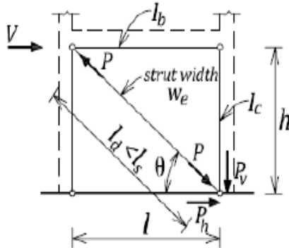
Fig. 5 Diagonal strut model, NBCC 2005 [21]
