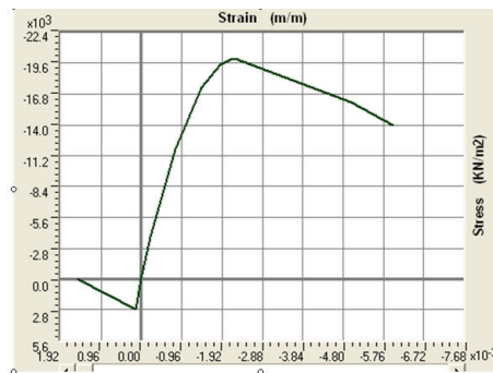
Fig. 11 (a) Stress-strain curve for concrete
