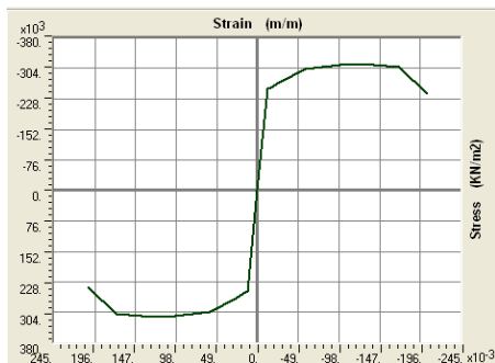
Fig. 11 (b) Stress-strain curve for steel bars
