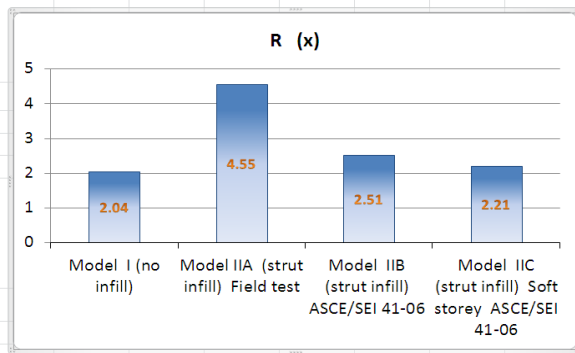
Fig. 18 (a) X - Direction
