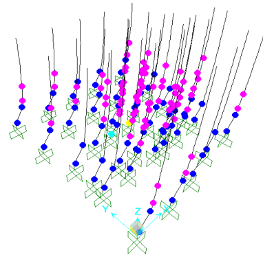
Fig. 12 (c) Model IIB (strut infill- ASCE/SEI 41)
