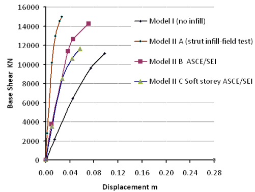
Fig. 14 (b) Static nonlinear analysis Y-Y
