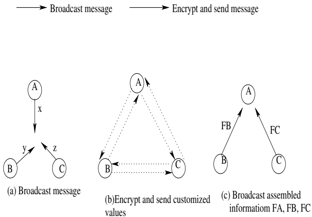
Fig. 2: Message Exchange.
