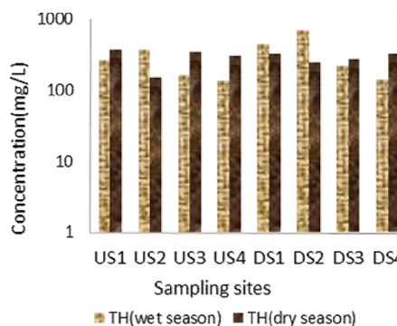
Fig. 3 Seasonal Variation of total hardness (TH) as CaCO 3 in Ga-Selati River
